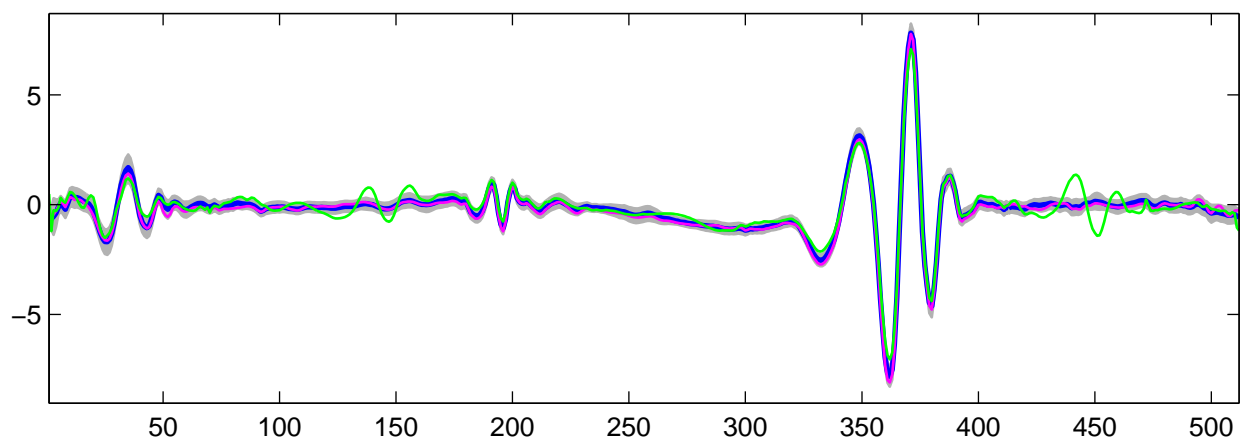
Estimated U_{30}(t) using R-WFMM: t_1 data, run 5
