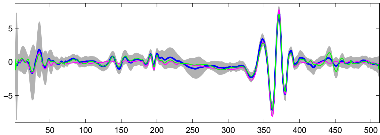
Estimated U_{30}(t) using G-WFMM: t_1 data, run 5
