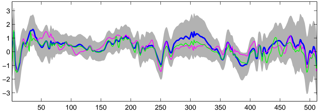
Estimated U_{30}(t) using G-WFMM: t_2 data, run 5
