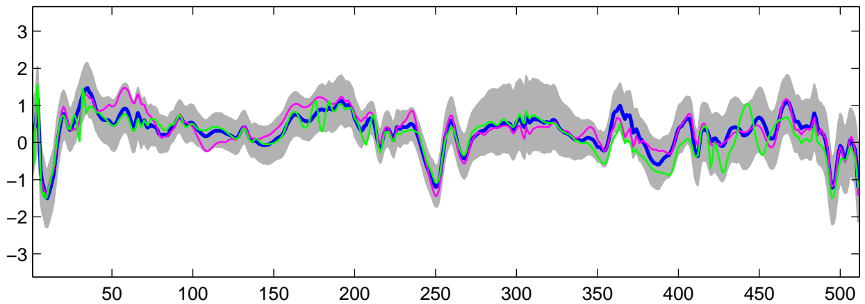
Estimated U_{30}(t) using R-WFMM: t_2 data, run 5
