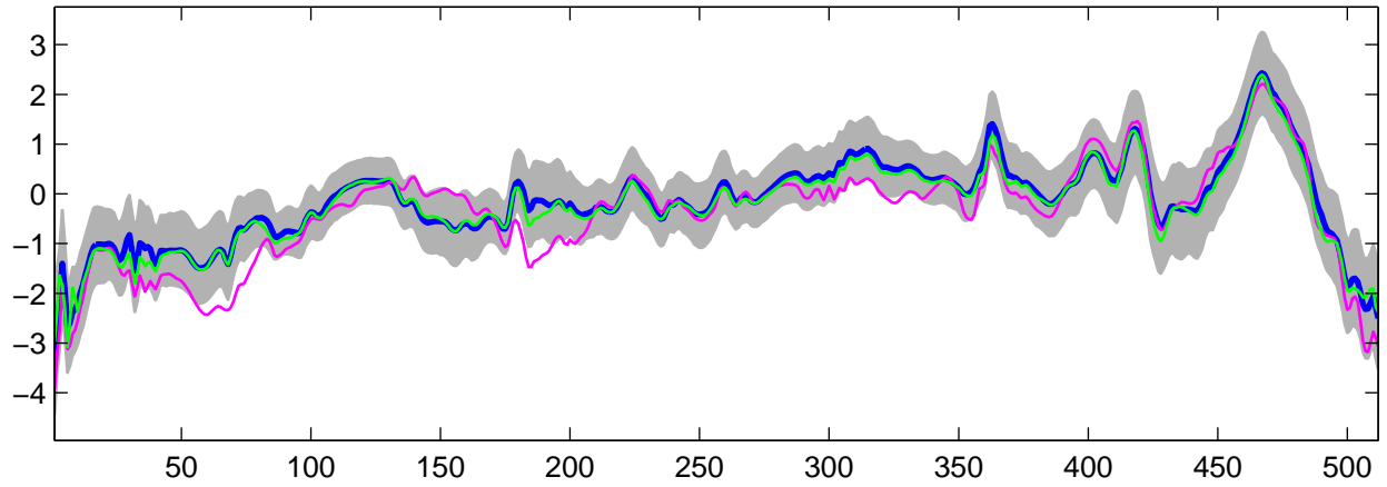
Estimated U_{30}(t) using G-WFMM: t_3 data, run 5
