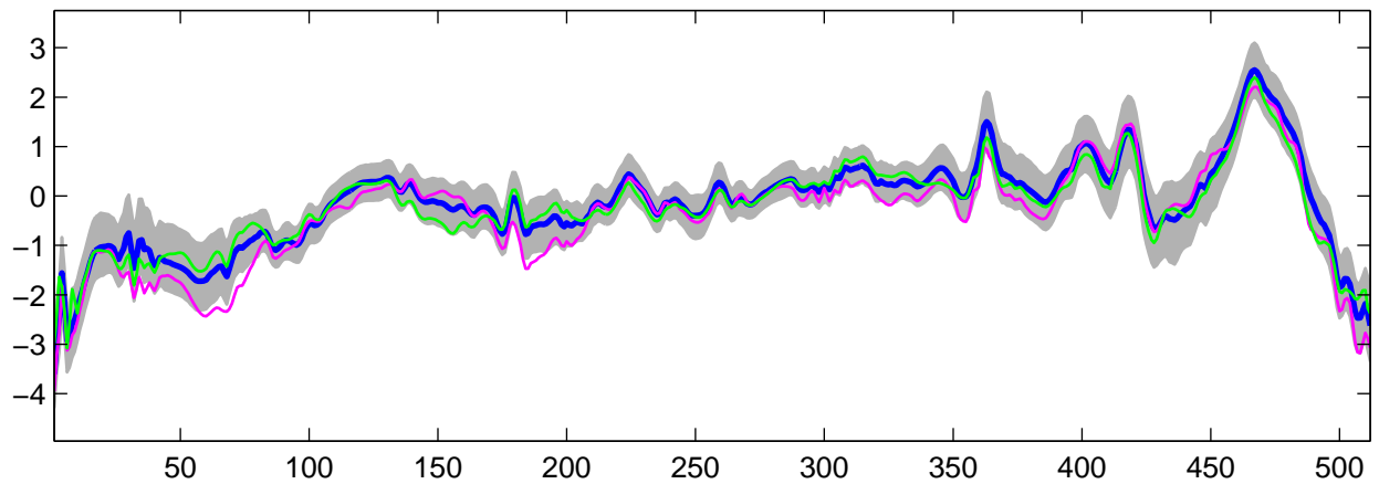
Estimated U_{30}(t) using R-WFMM: t_3 data, run 5
