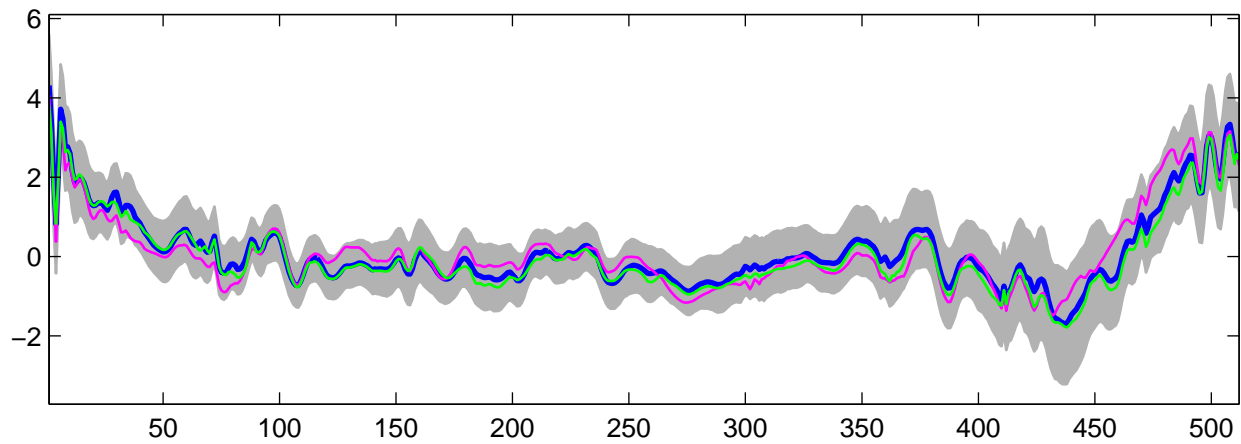
Estimated U_{31}(t) using G-WFMM: DE data, run 5
