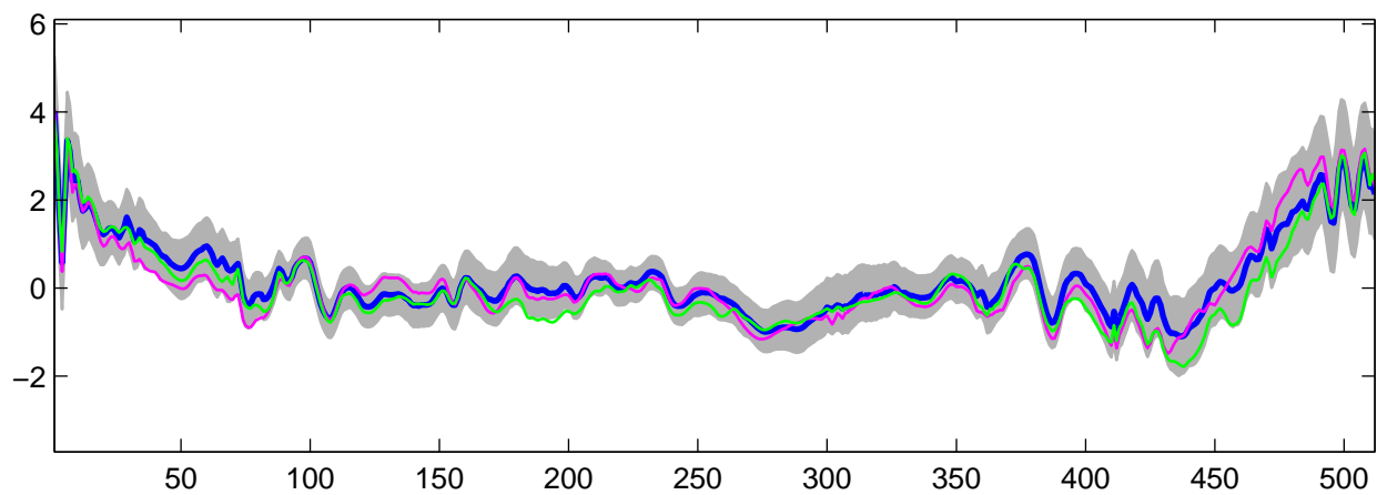
Estimated U_{31}(t) using R-WFMM: DE data, run 5
