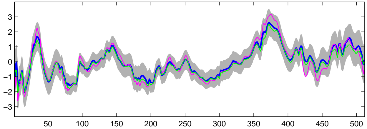
Estimated U_{31}(t) using G-WFMM: Normal data, run 5
