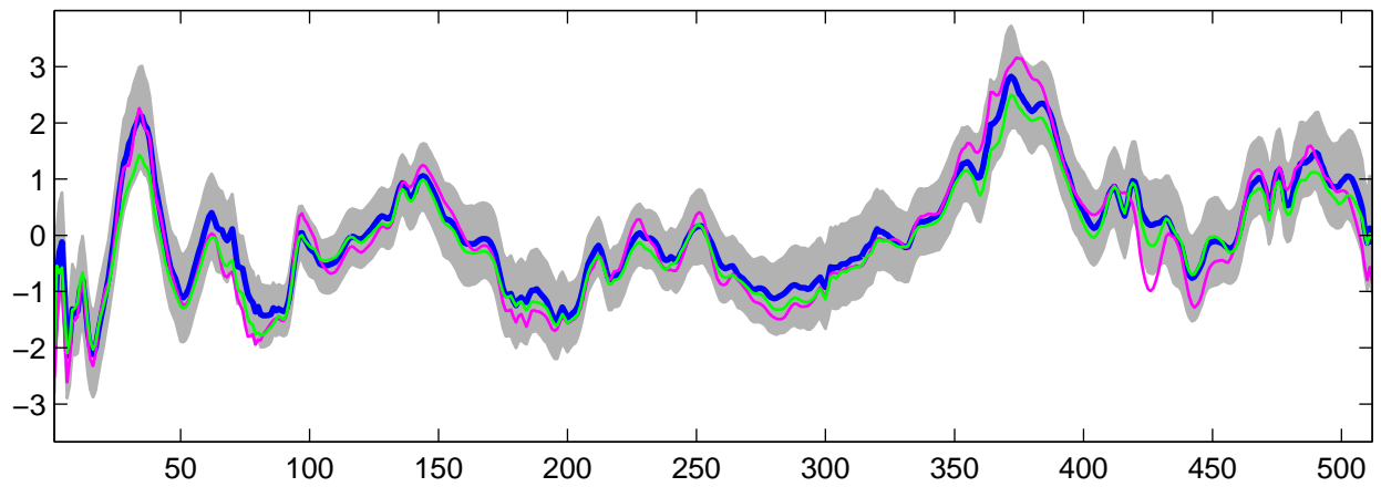
Estimated U_{31}(t) using R-WFMM: Normal data, run 5
