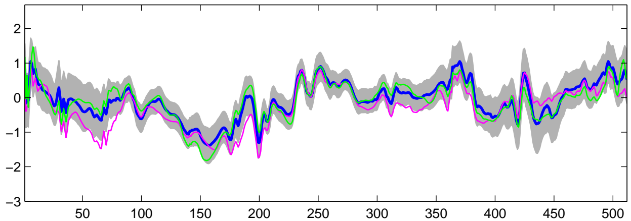
Estimated U_{31}(t) using R-WFMM: t_3 data, run 5
