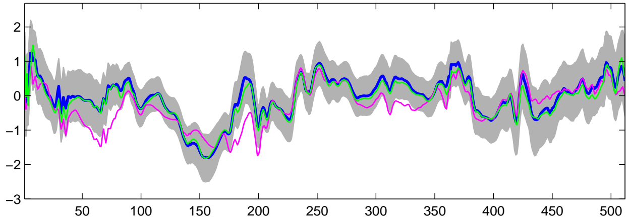
Estimated U_{31}(t) using G-WFMM: t_3 data, run 5
