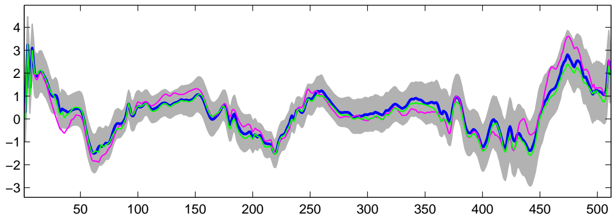
Estimated U_{32}(t) using G-WFMM: DE data, run 5
