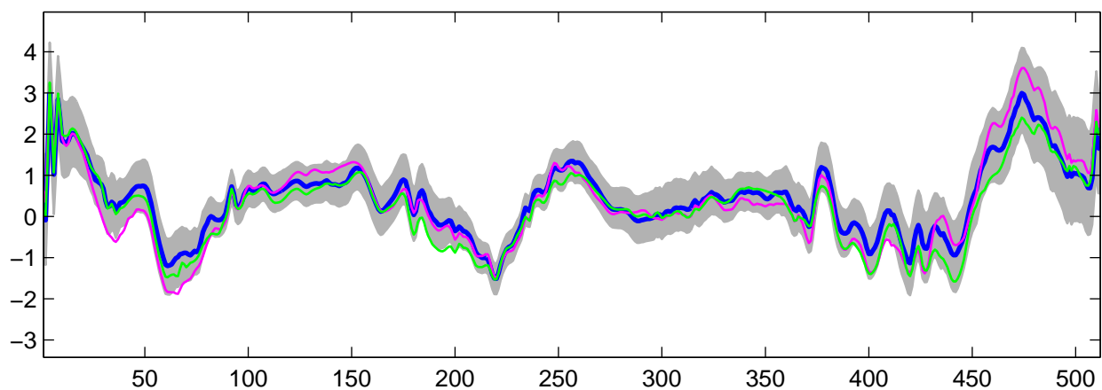
Estimated U_{32}(t) using R-WFMM: DE data, run 5
