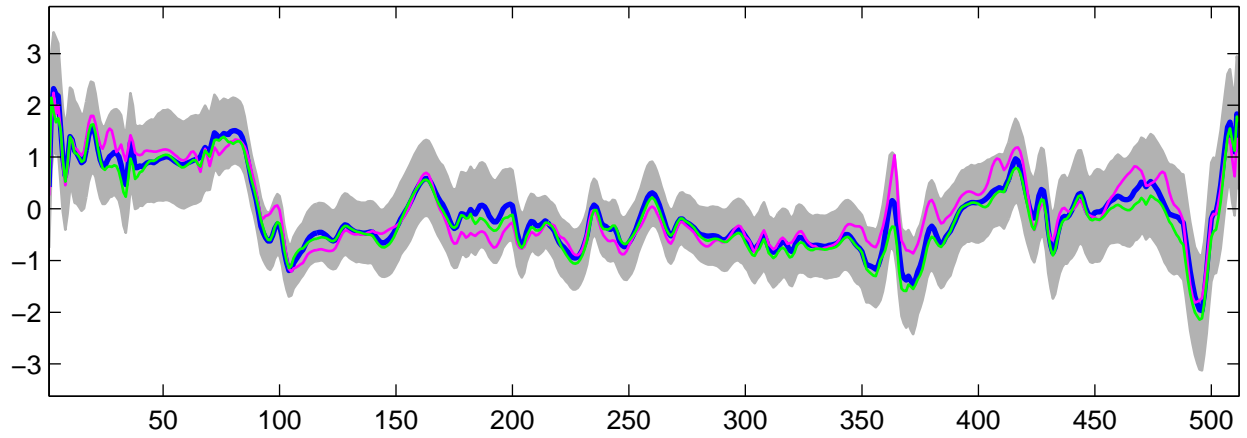
Estimated U_{32}(t) using G-WFMM: Normal data, run 5
