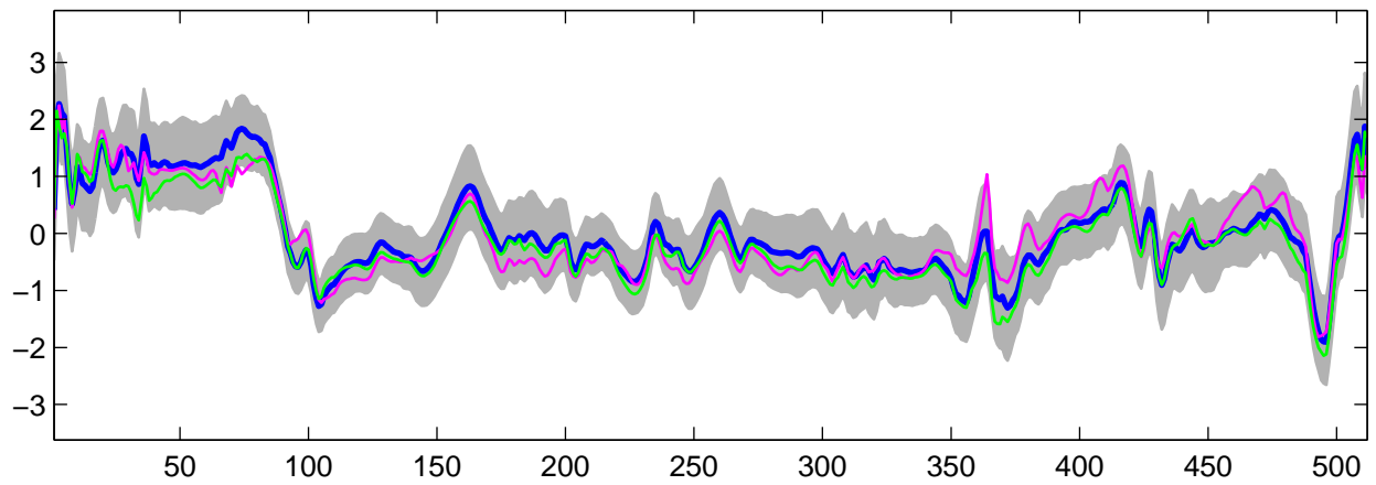
Estimated U_{32}(t) using R-WFMM: Normal data, run 5
