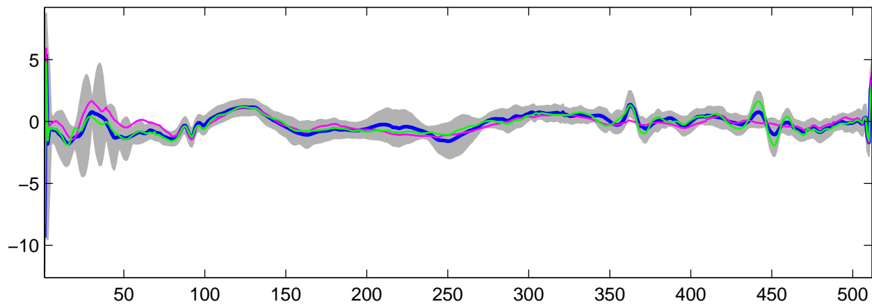
Estimated U_{32}(t) using G-WFMM: t_1 data, run 5
