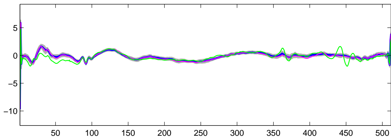
Estimated U_{32}(t) using R-WFMM: t_1 data, run 5
