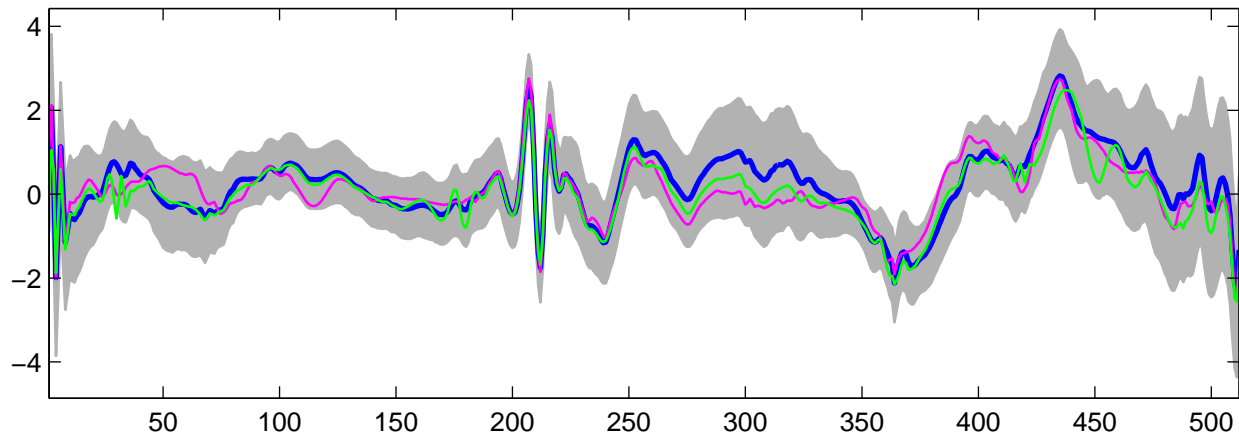
Estimated U_{32}(t) using G-WFMM: t_2 data, run 5
