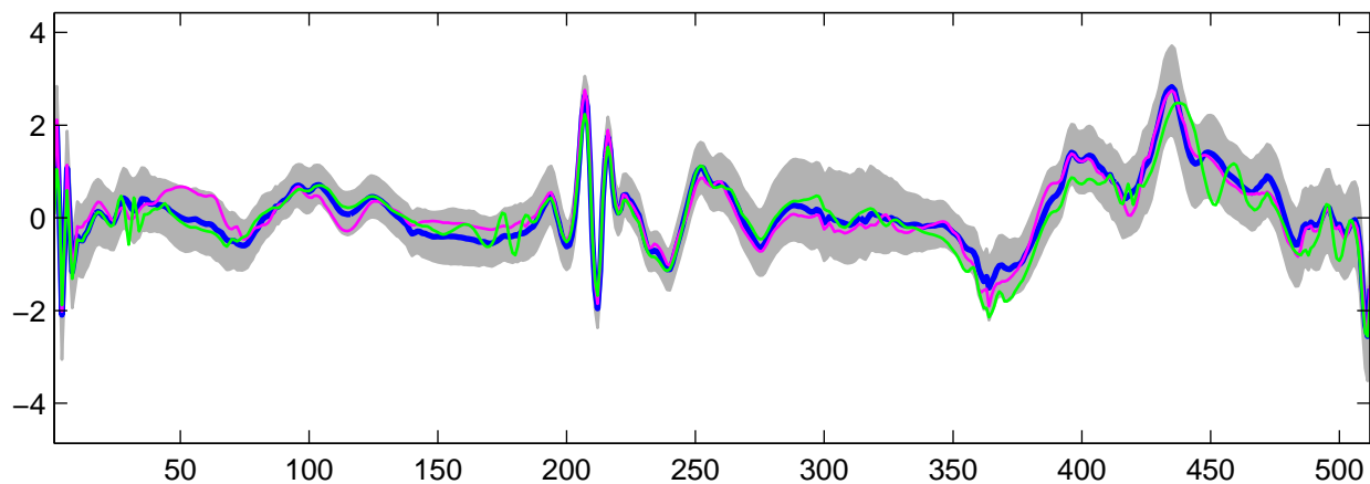
Estimated U_{32}(t) using R-WFMM: t_2 data, run 5
