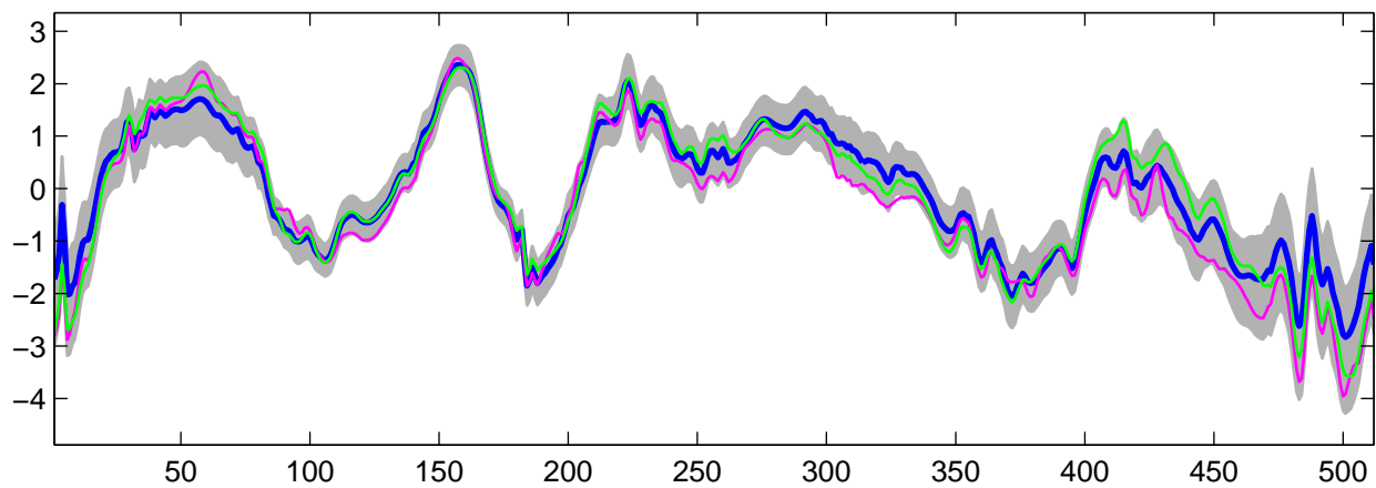
Estimated U_3(t) using R-WFMM: DE data, run 5
