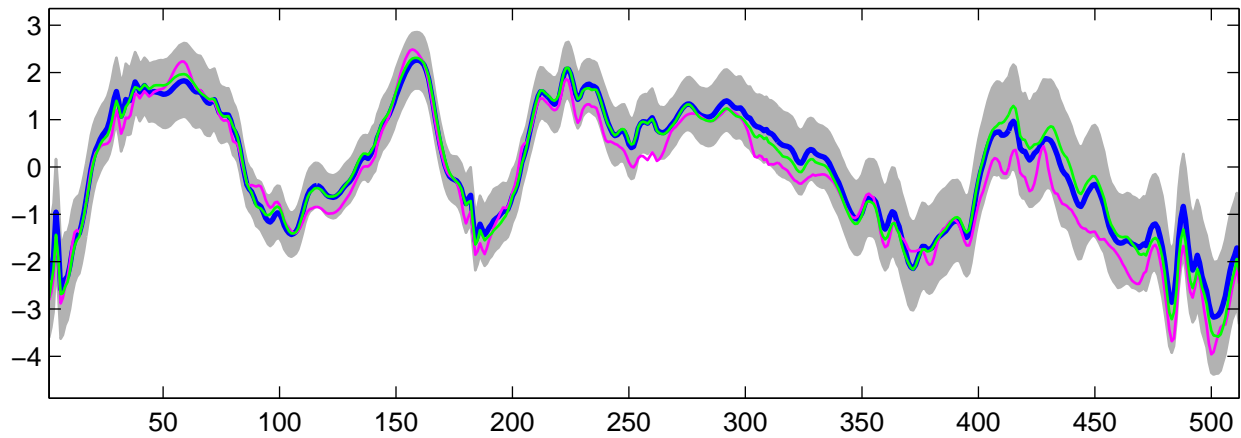
Estimated U_3(t) using G-WFMM: DE data, run 5
