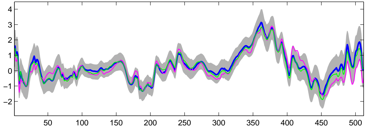
Estimated U_3(t) using G-WFMM: Normal data, run 5
