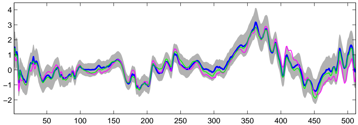
Estimated U_3(t) using R-WFMM: Normal data, run 5
