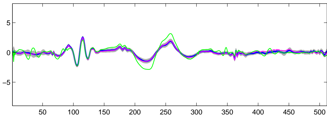
Estimated U_3(t) using R-WFMM: t_1 data, run 5
