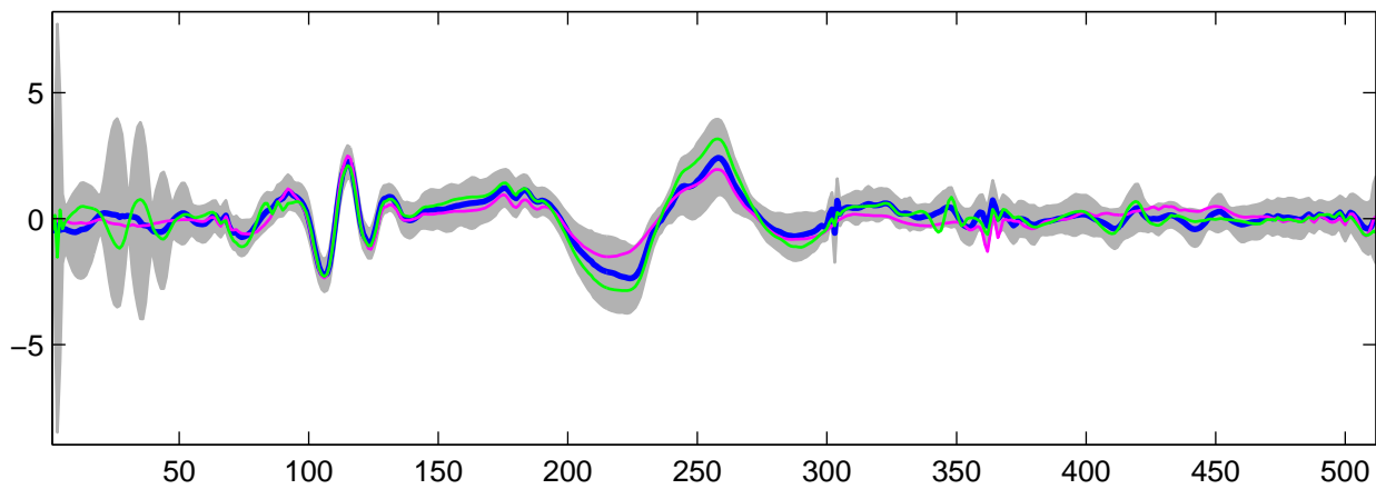
Estimated U_3(t) using G-WFMM: t_1 data, run 5
