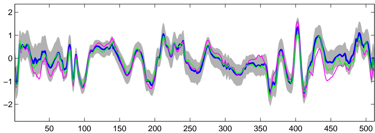
Estimated U_3(t) using R-WFMM: t_3 data, run 5
