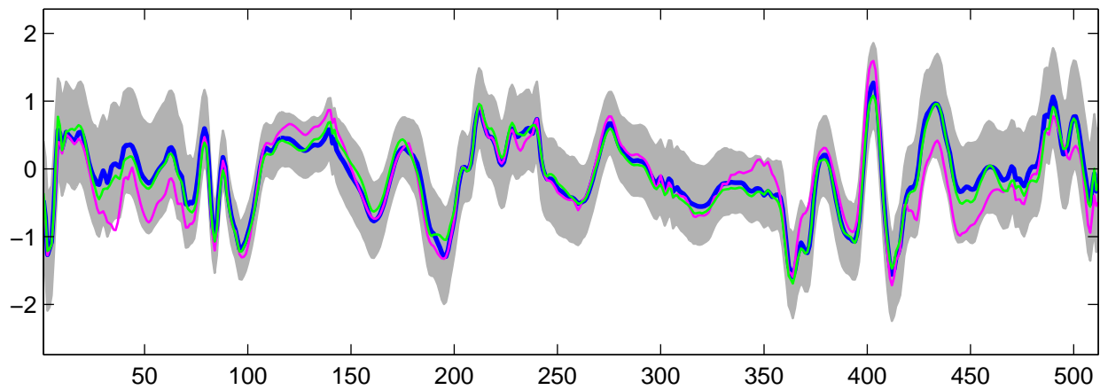
Estimated U_3(t) using G-WFMM: t_3 data, run 5
