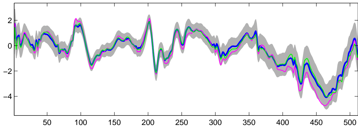
Estimated U_4(t) using G-WFMM: DE data, run 5
