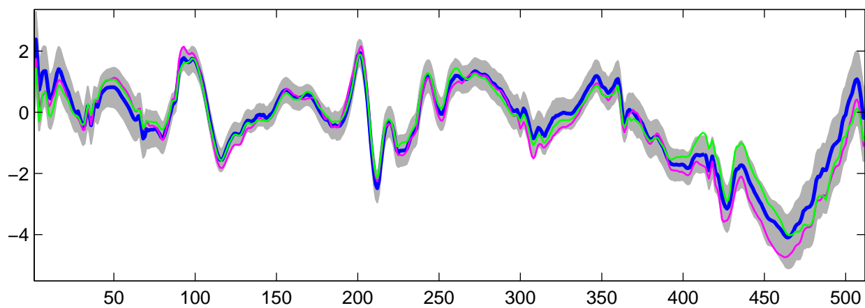
Estimated U_4(t) using R-WFMM: DE data, run 5
