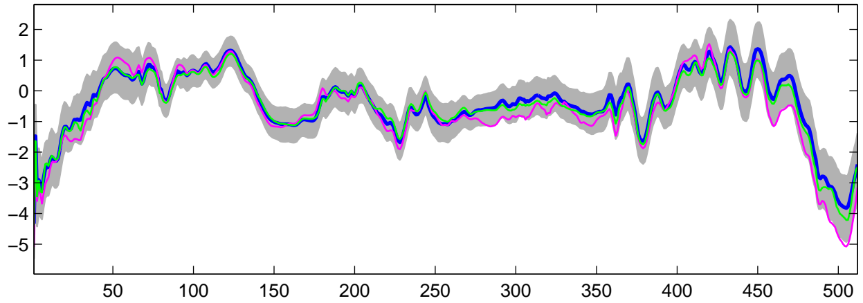
Estimated U_4(t) using G-WFMM: Normal data, run 5
