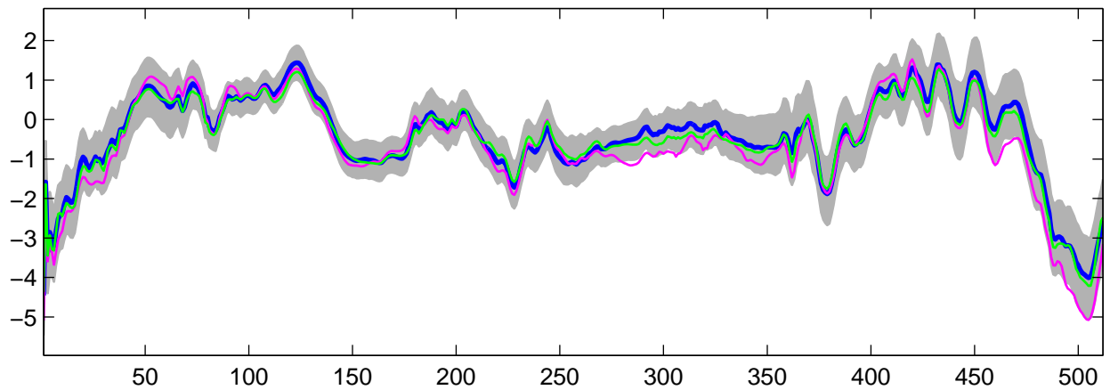
Estimated U_4(t) using R-WFMM: Normal data, run 5
