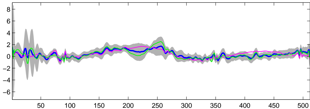
Estimated U_4(t) using G-WFMM: t_1 data, run 5
