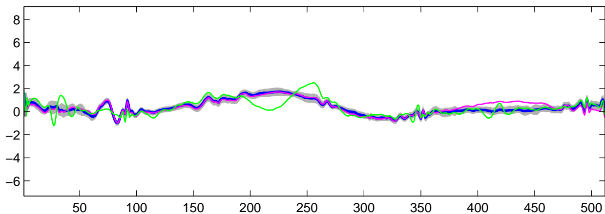
Estimated U_4(t) using R-WFMM: t_1 data, run 5
