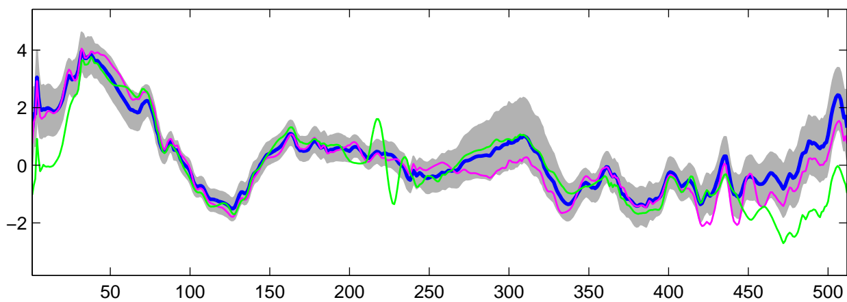
Estimated U_4(t) using R-WFMM: t_2 data, run 5
