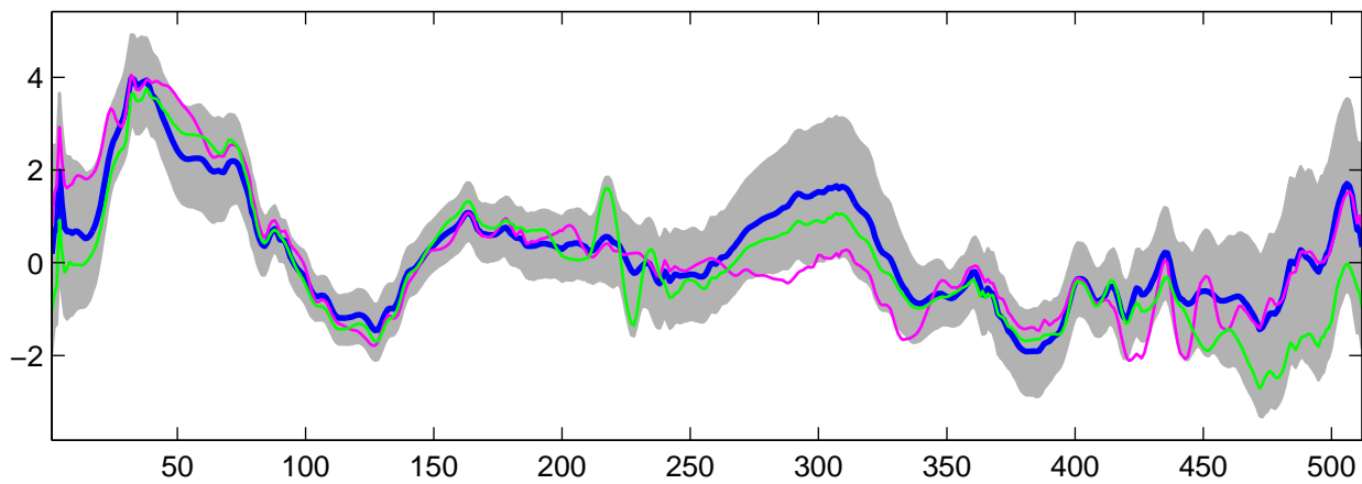
Estimated U_4(t) using G-WFMM: t_2 data, run 5
