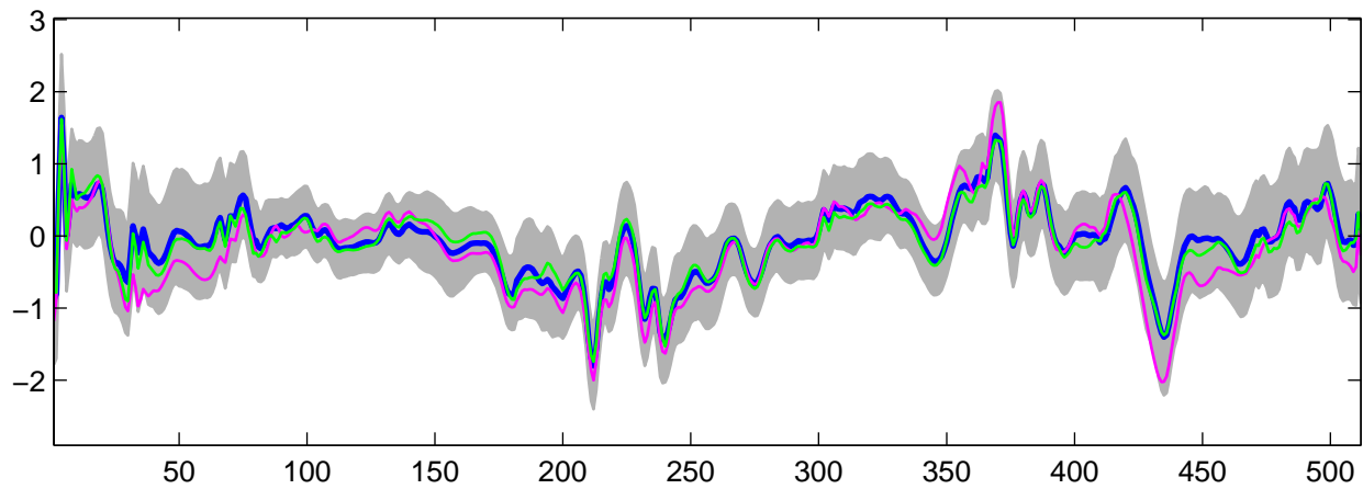
Estimated U_4(t) using G-WFMM: t_3 data, run 5
