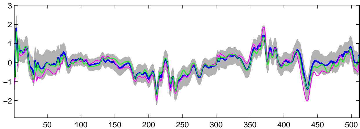
Estimated U_4(t) using R-WFMM: t_3 data, run 5
