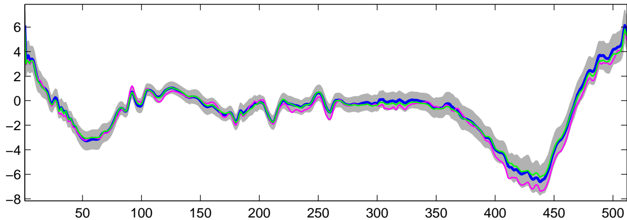
Estimated U_5(t) using G-WFMM: DE data, run 5
