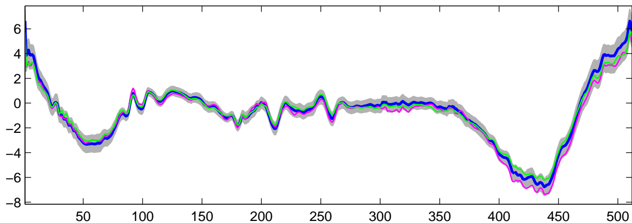
Estimated U_5(t) using R-WFMM: DE data, run 5
