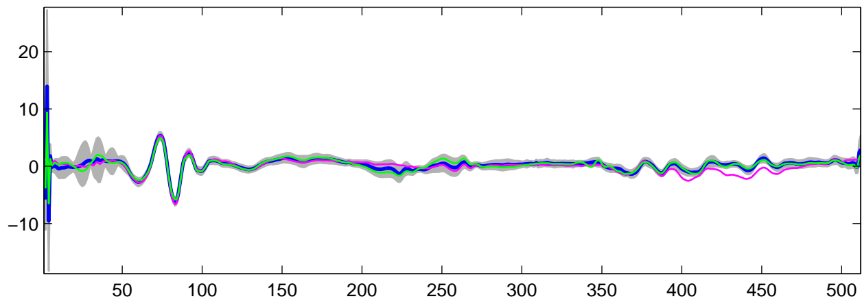
Estimated U_5(t) using G-WFMM: t_1 data, run 5
