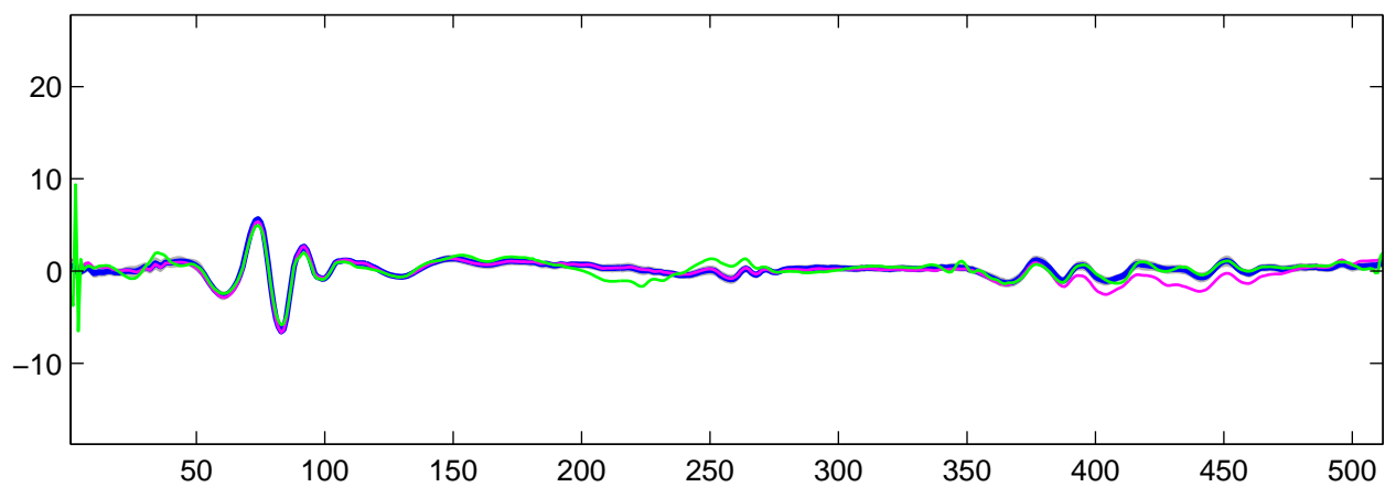
Estimated U_5(t) using R-WFMM: t_1 data, run 5
