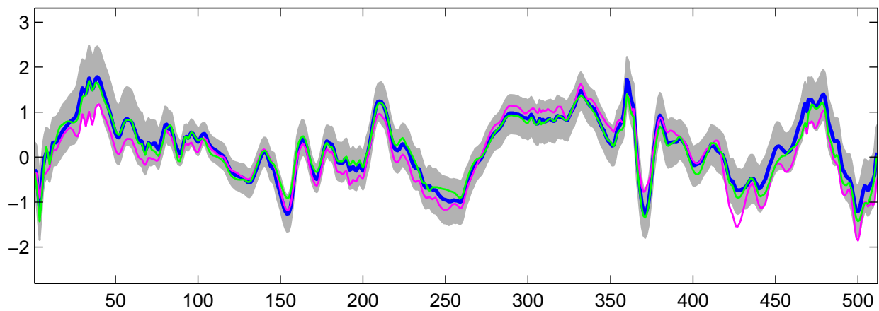
Estimated U_5(t) using R-WFMM: t_3 data, run 5
