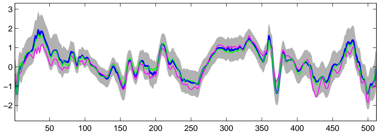
Estimated U_5(t) using G-WFMM: t_3 data, run 5
