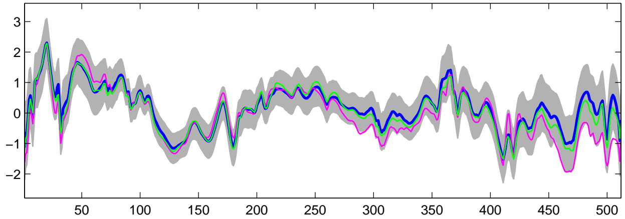
Estimated U_6(t) using G-WFMM: Normal data, run 5
