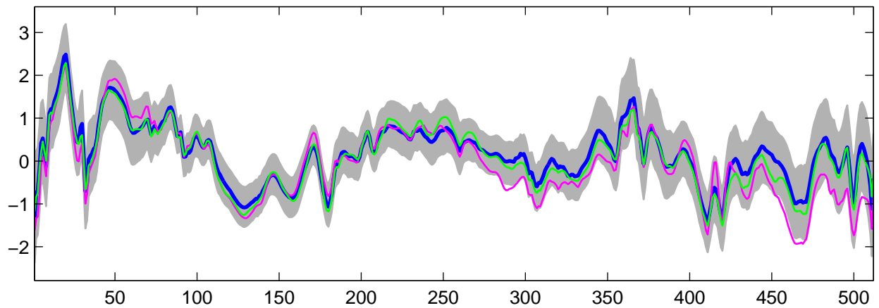
Estimated U_6(t) using R-WFMM: Normal data, run 5
