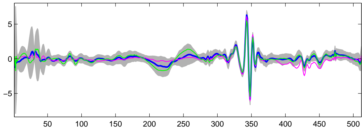
Estimated U_6(t) using G-WFMM: t_1 data, run 5
