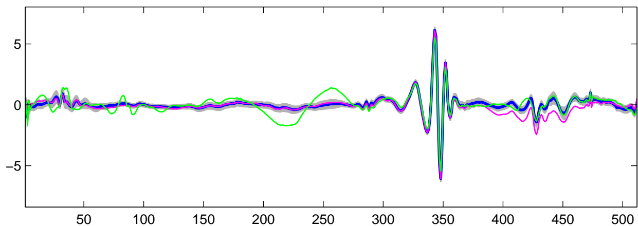
Estimated U_6(t) using R-WFMM: t_1 data, run 5
