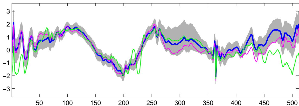
Estimated U_6(t) using R-WFMM: t_2 data, run 5
