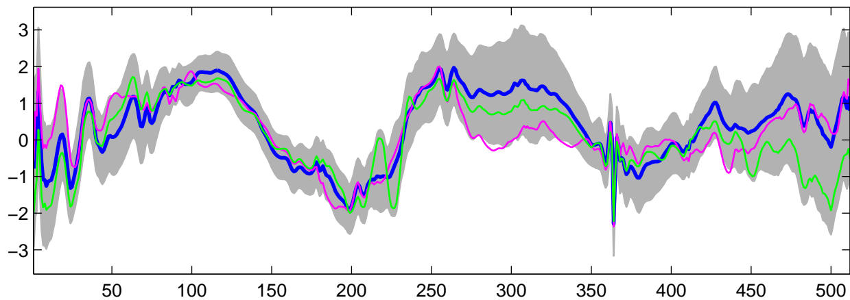
Estimated U_6(t) using G-WFMM: t_2 data, run 5
