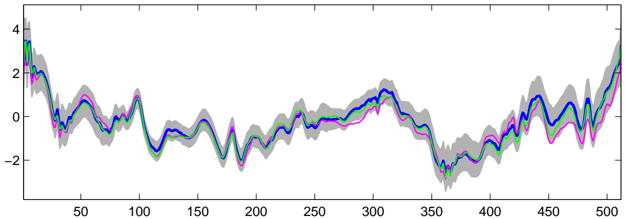
Estimated U_7(t) using R-WFMM: Normal data, run 5
