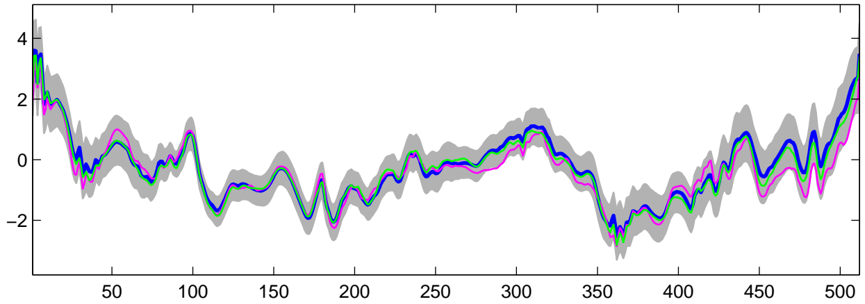
Estimated U_7(t) using G-WFMM: Normal data, run 5
