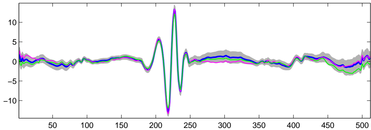
Estimated U_7(t) using G-WFMM: t_2 data, run 5
