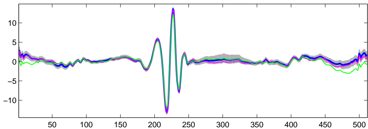
Estimated U_7(t) using R-WFMM: t_2 data, run 5
