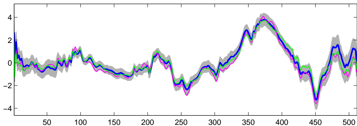
Estimated U_g(t) using R-WFMM: DE data, run 5
