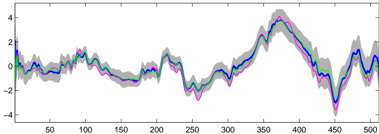
Estimated U_g(t) using G-WFMM: DE data, run 5
