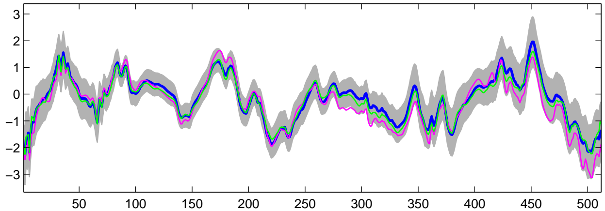
Estimated U_g(t) using R-WFMM: Normal data, run 5
