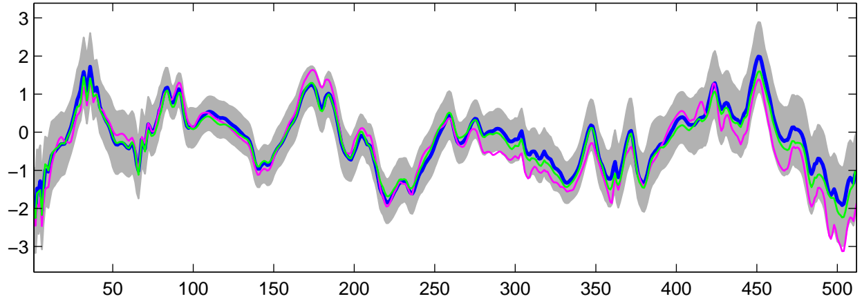
Estimated U_g(t) using G-WFMM: Normal data, run 5
