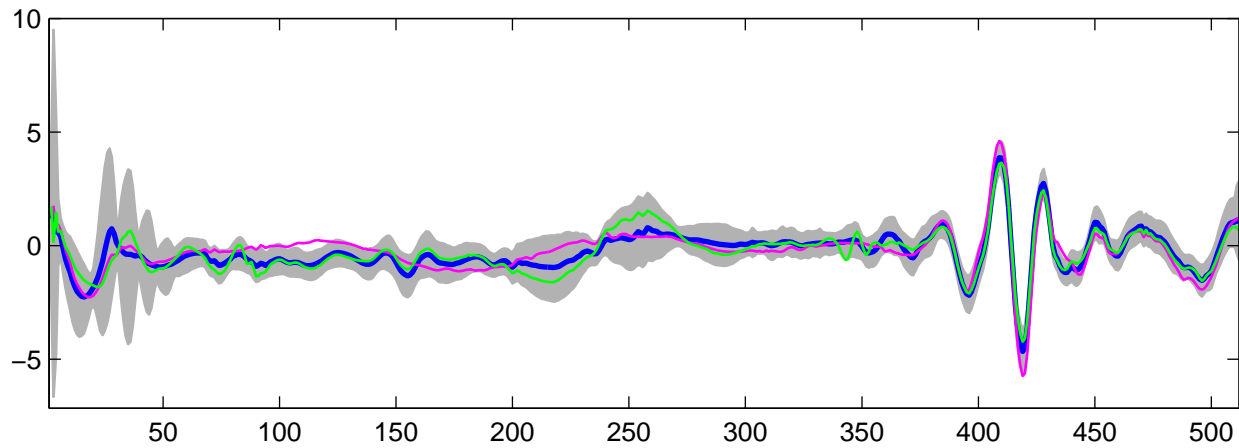
Estimated U_g(t) using G-WFMM: t_1 data, run 5
