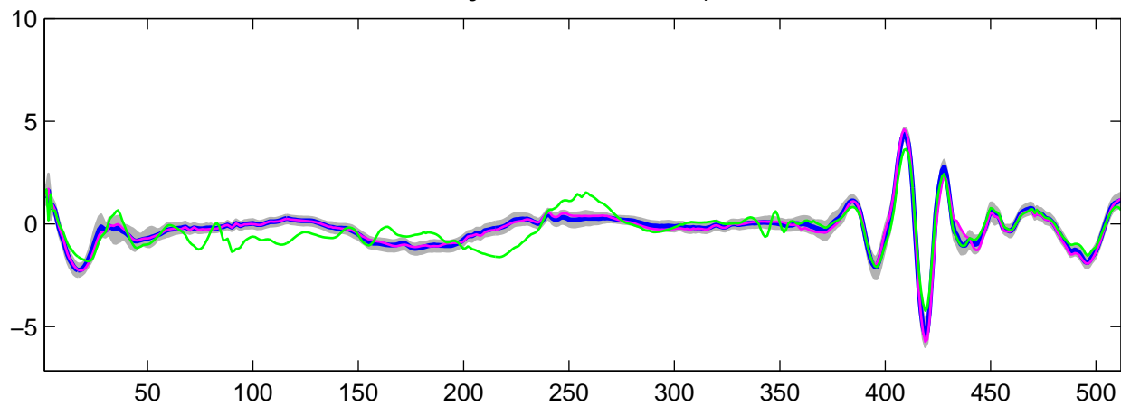
Estimated U_g(t) using R-WFMM: t_1 data, run 5
