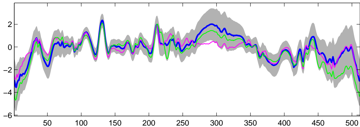
Estimated U_8(t) using G-WFMM: t_2 data, run 5
