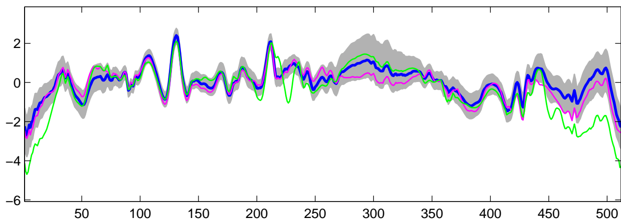
Estimated U_8(t) using R-WFMM: t_2 data, run 5
