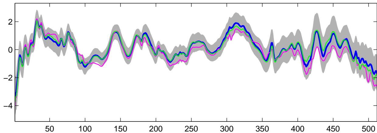
Estimated U_\theta(t) using G-WFMM: DE data, run 5
