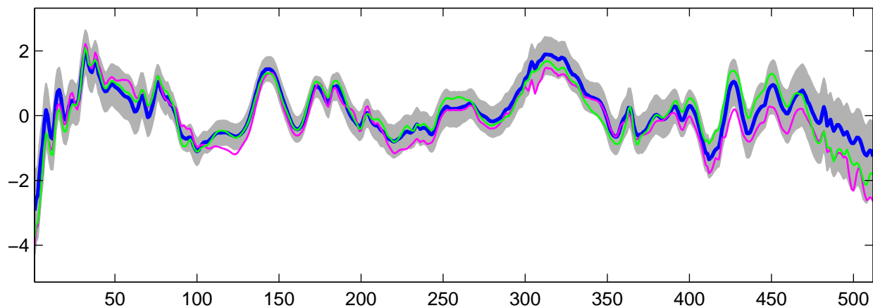
Estimated U_\theta(t) using R-WFMM: DE data, run 5
