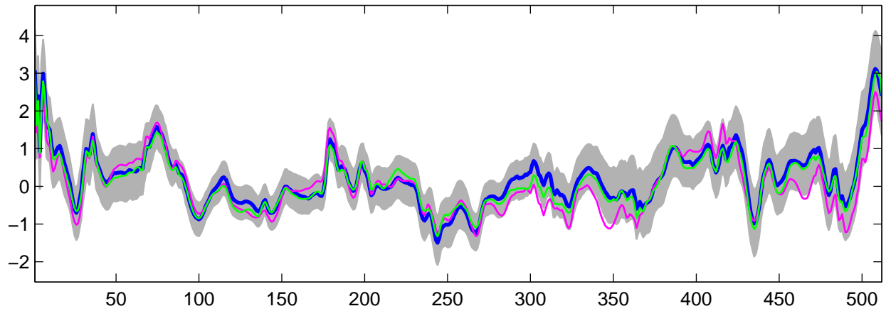
Estimated U_{\theta}(t) using R-WFMM: Normal data, run 5
