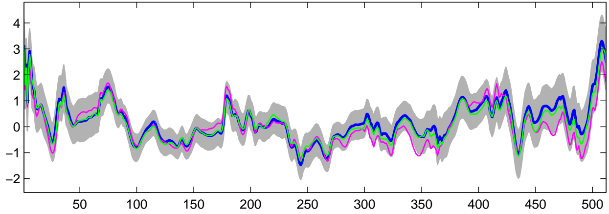
Estimated U_{\theta}(t) using G-WFMM: Normal data, run 5
