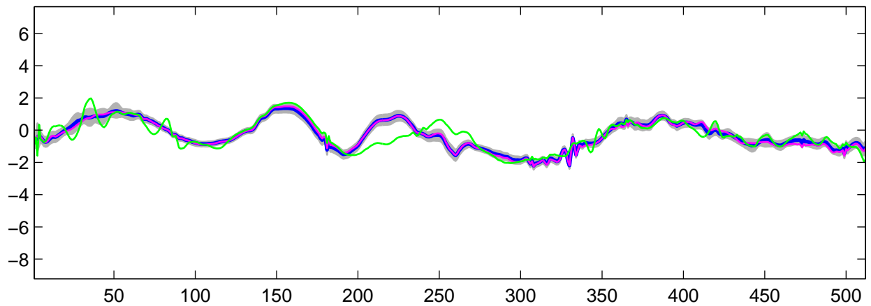
Estimated U_{\theta}(t) using R-WFMM: t_1 data, run 5
