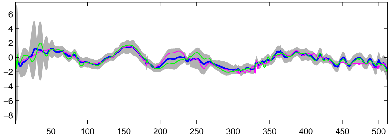
Estimated U_{\theta}(t) using G-WFMM: t_1 data, run 5
