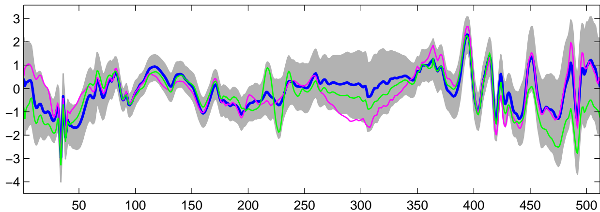
Estimated U_9(t) using G-WFMM: t_2 data, run 5
