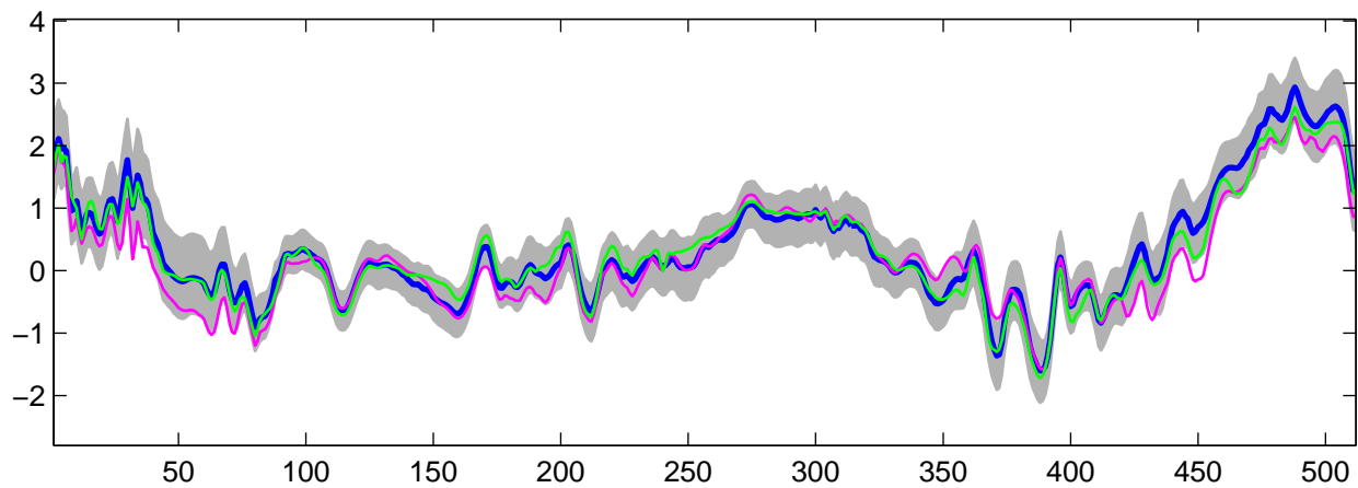
Estimated U_\theta(t) using R-WFMM: t_3 data, run 5
