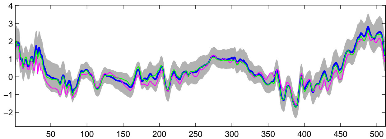
Estimated U_\theta(t) using G-WFMM: t_3 data, run 5
