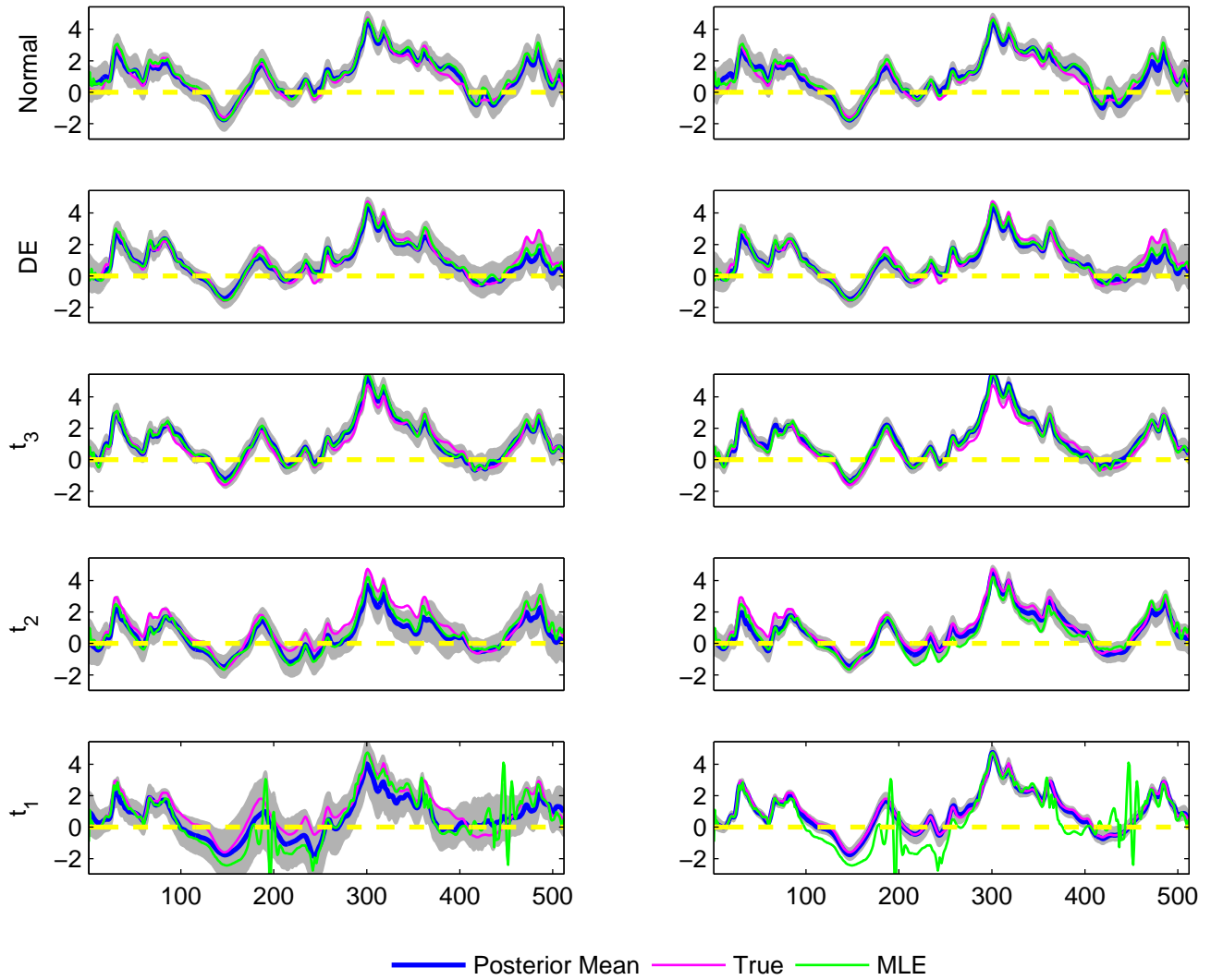
The estimated B_2(t) for 5 simulated datasets, simulation run 6
