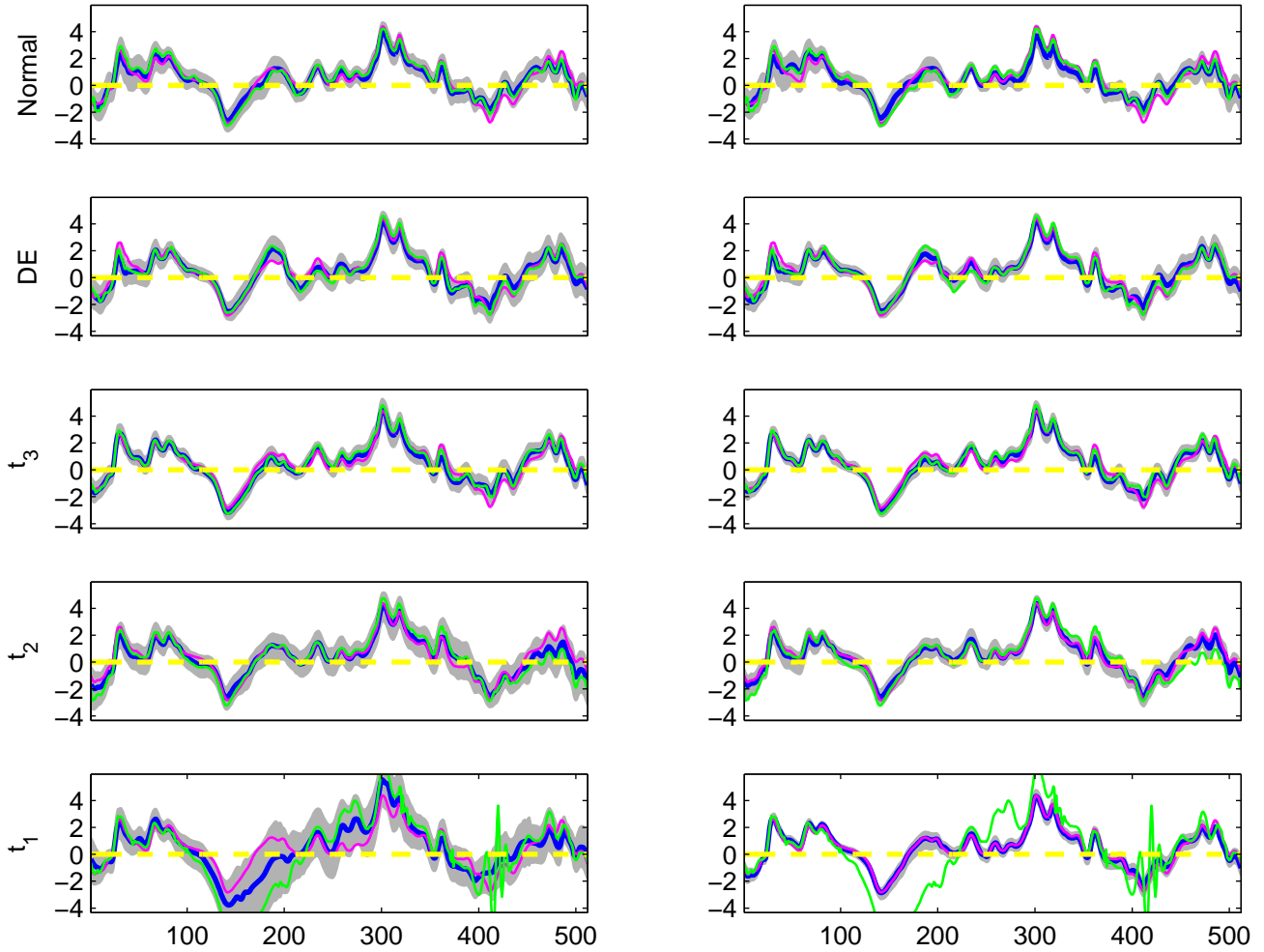
The estimated B_3(t) for 5 simulated datasets, simulation run 6 G-WFMM R-WFMM
