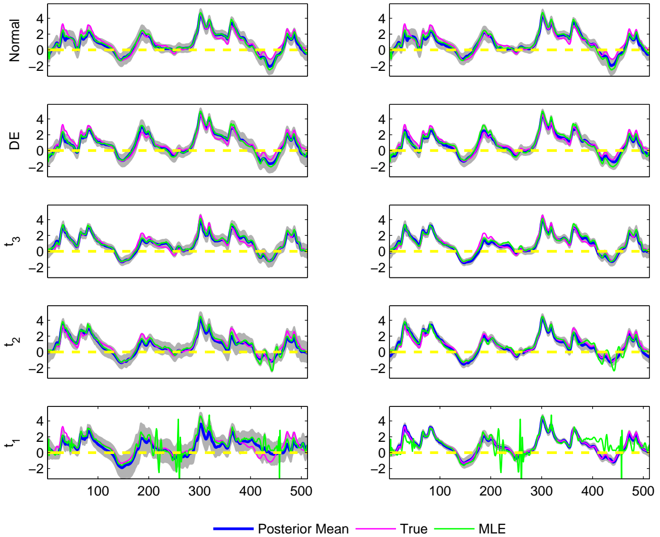
The estimated B_4(t) for 5 simulated datasets, simulation run 6
