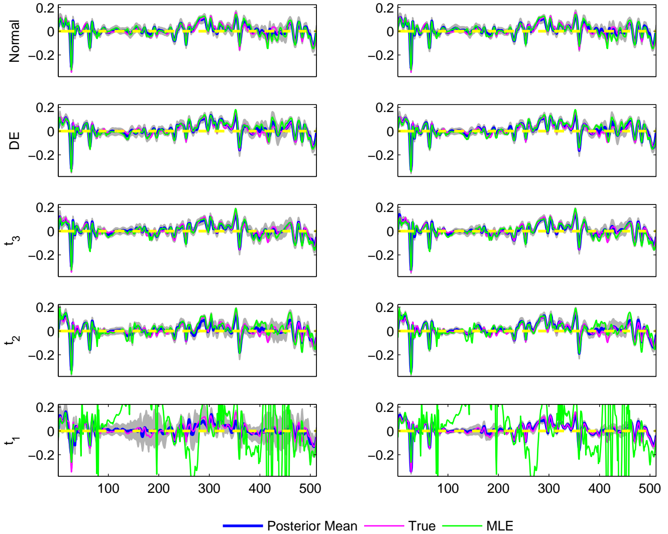
The estimated B_5(t) for 5 simulated datasets, simulation run 6
