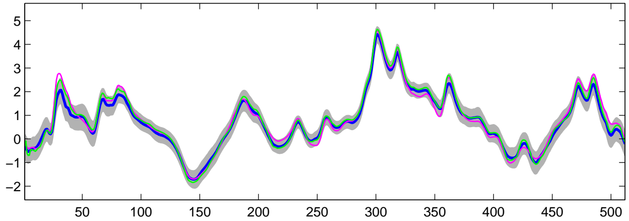
Estimated C_0(t) using G-WFMM: Normal data, run 6
