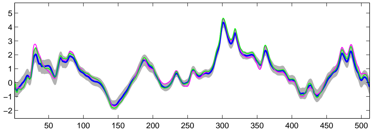
Estimated C_0(t) using R-WFMM: Normal data, run 6
