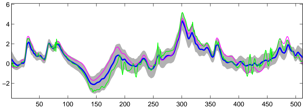
Estimated C_0(t) using G-WFMM: t_1 data, run 6
