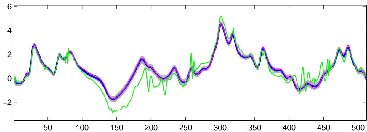
Estimated C_0(t) using R-WFMM: t_1 data, run 6
