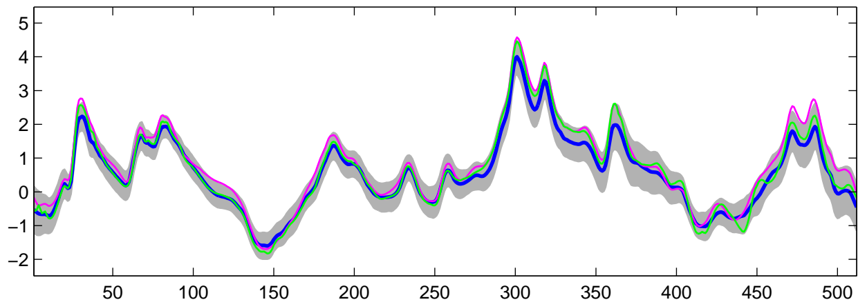
Estimated C_0(t) using G-WFMM: t_2 data, run 6
