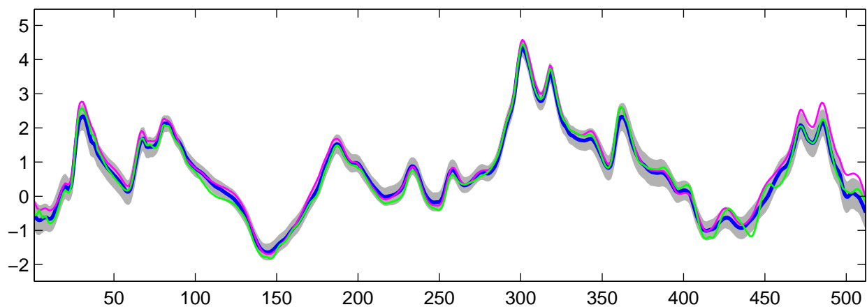
Estimated C_0(t) using R-WFMM: t_2 data, run 6
