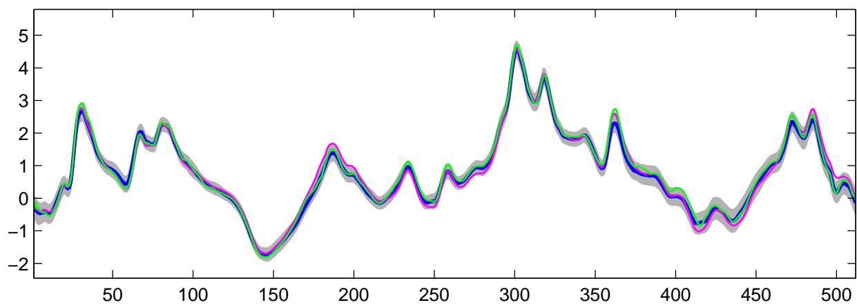
Estimated C_0(t) using R-WFMM: t_3 data, run 6
