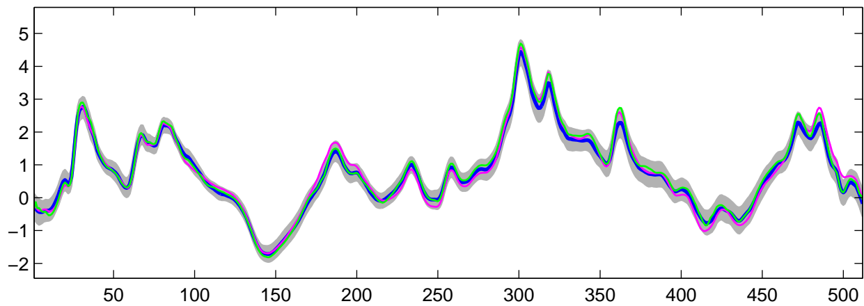
Estimated C_0(t) using G-WFMM: t_3 data, run 6
