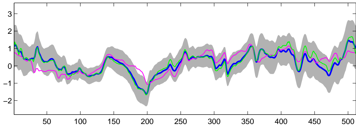
Estimated C_1(t) using G-WFMM: DE data, run 6
