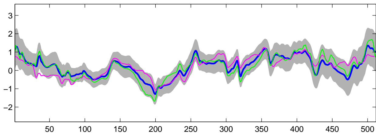
Estimated C_1(t) using R-WFMM: DE data, run 6
