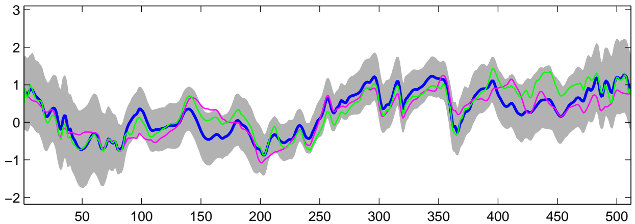
Estimated C_1(t) using R-WFMM: Normal data, run 6
