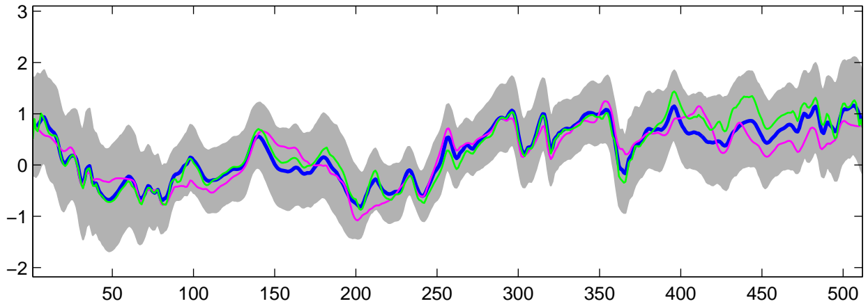
Estimated C_1(t) using G-WFMM: Normal data, run 6
