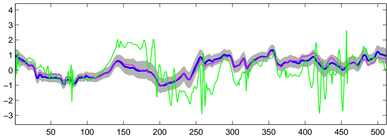
Estimated C_1(t) using R-WFMM: t_1 data, run 6
