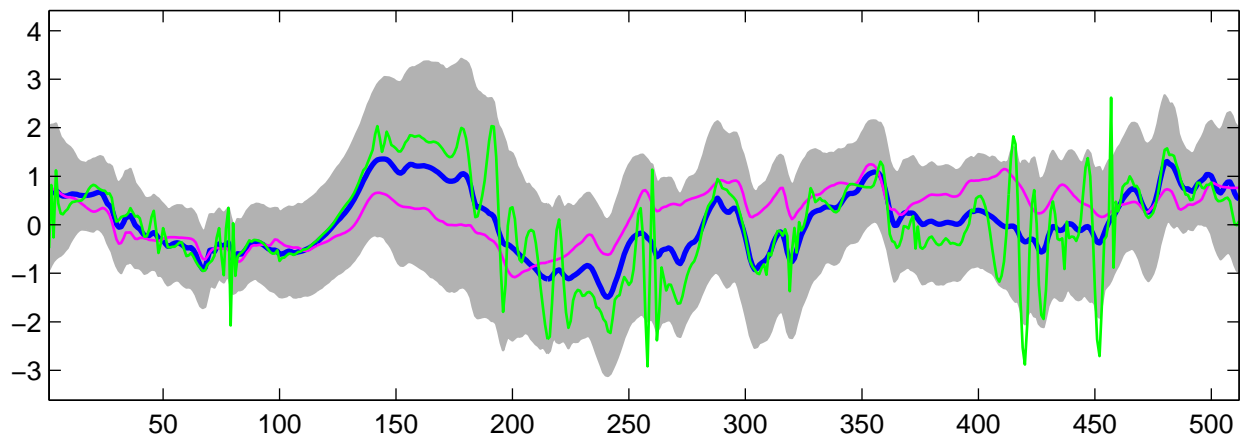
Estimated C_1(t) using G-WFMM: t_1 data, run 6
