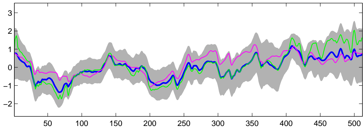
Estimated C_1(t) using G-WFMM: t_2 data, run 6
