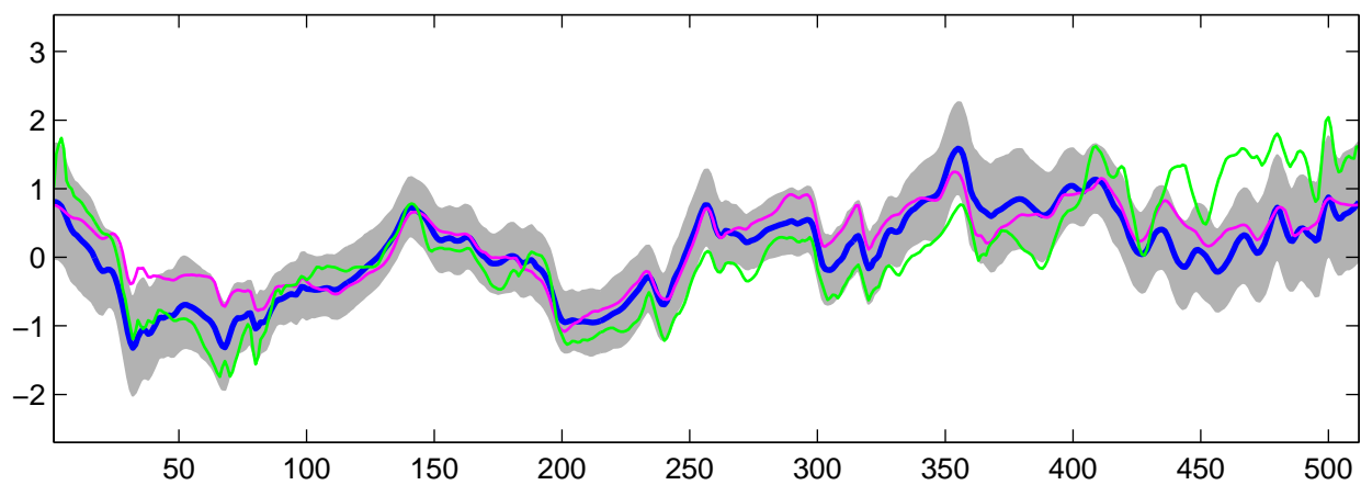
Estimated C_1(t) using R-WFMM: t_2 data, run 6
