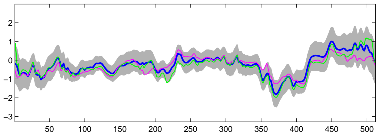
Estimated C_2(t) using R-WFMM: DE data, run 6
