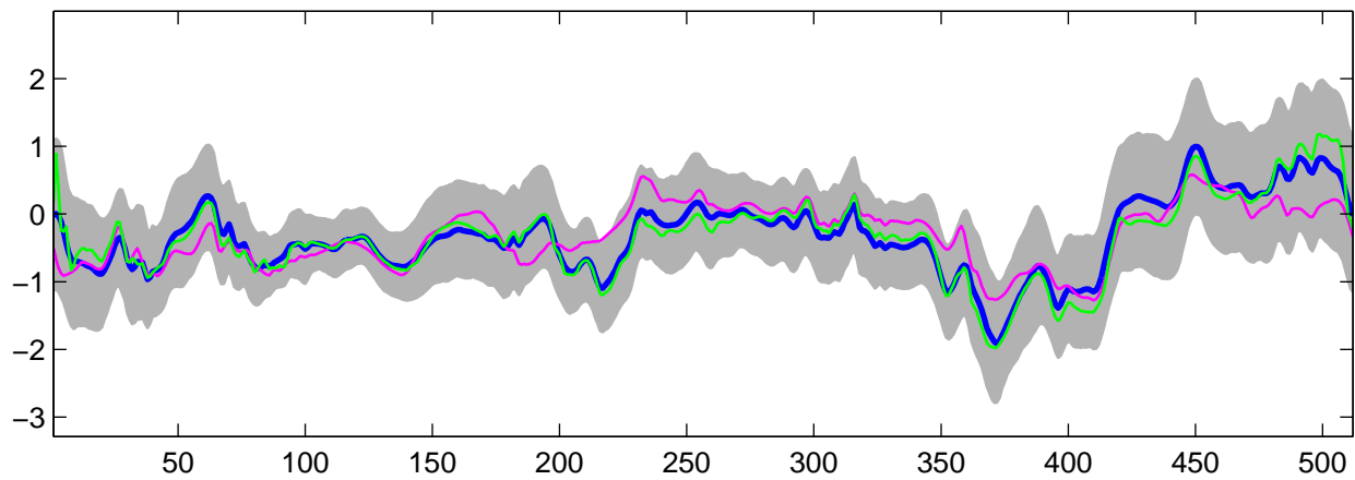
Estimated C_2(t) using G-WFMM: DE data, run 6
