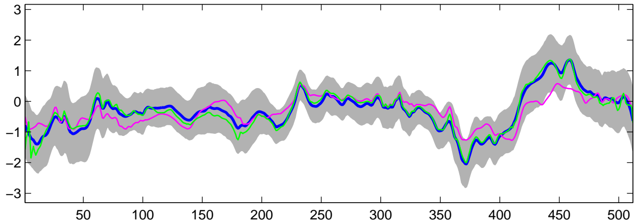
Estimated C_2(t) using G-WFMM: Normal data, run 6
