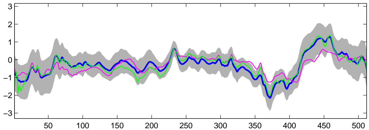
Estimated C_2(t) using R-WFMM: Normal data, run 6
